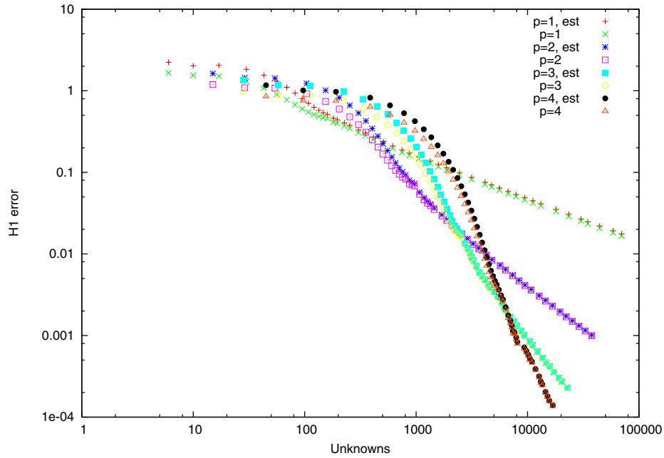
Figure 2. Results for L-shaped domain. The equilibration is performed with BDM^{p+1} elements. are
