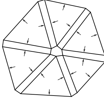
FIGURE 5. Slim rectangles in the sense of Remark 6.
