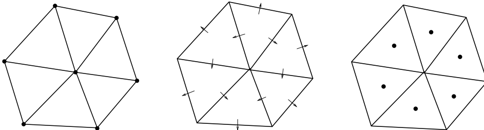
FIGURE 2. Classical finite element spaces in the sequence (3.3).
