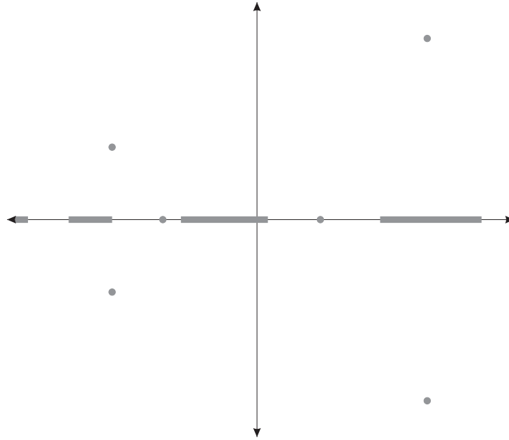
Figure 3.1: \sigma(A)
