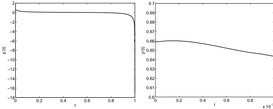
Figure 5: Derivative of the numerical solution of (4.3), (4.4), (4.5) for a_0 = 1 , b_0 = 2 , \gamma = \frac{3}{2} . Left graph: p'(t) , t \in [0, 1] ; Right graph: p'(t) , t \in [0, 10^{-3}] .
