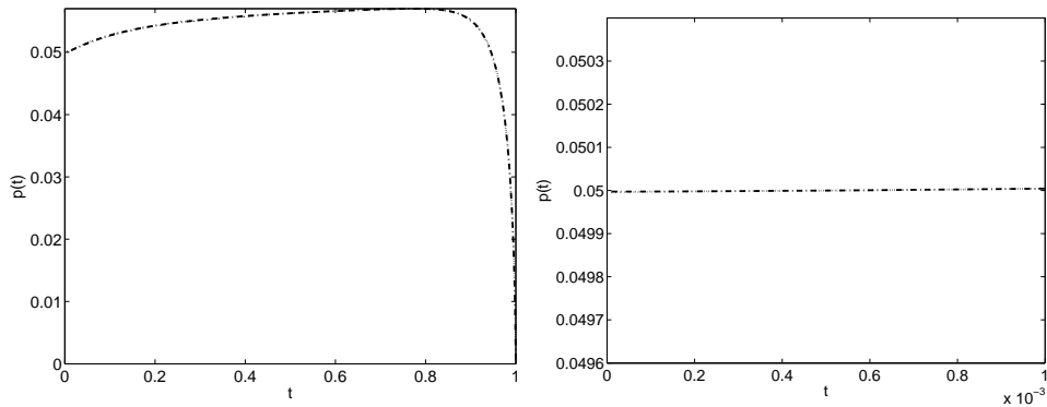
Figure 3: Figures (1) and (2) shown together in one graph. Dashed-dotted line: Solution of the first formulation (4.1), (4.2). Dotted line: Solution of the second formulation (4.3), (4.4), (4.5).
