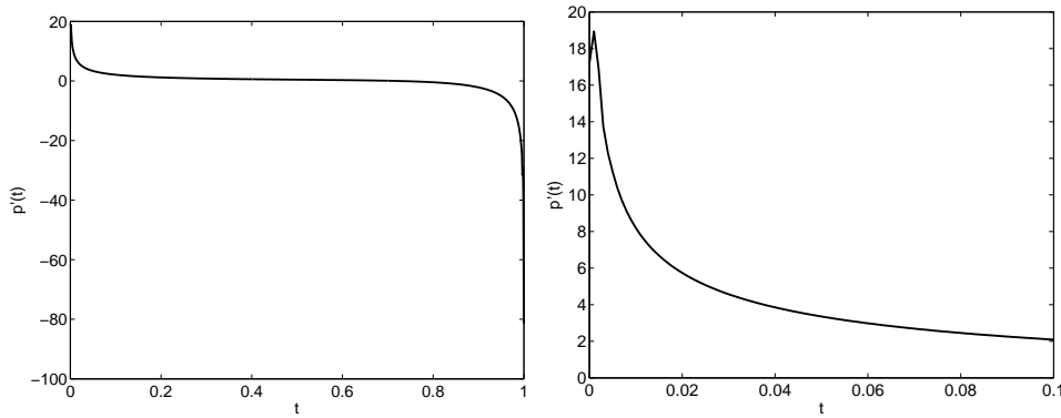
Figure 7: Derivative of the numerical solution of (4.3), (4.4), (4.5) for a_0 = 1 , b_0 = 2 , \gamma = 1.4 . Left graph: p'(t) , t \in [0, 1] ; Right graph: p'(t) , t \in [0, 10^{-1}] .
