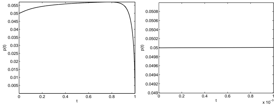
Figure 2: Numerical solution of (4.3), (4.4), (4.5) for a_0 = 2 , b_0 = 3 , \gamma = 1.8 . Left graph: p(t) , t \in [0, 1] ; Right graph: p(t) , t \in [0, 10^{-3}] .
