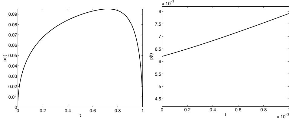
Figure 6: Numerical solution of (4.3), (4.4), (4.5) for a_0 = 1 , b_0 = 2 , \gamma = 1.4 . Left graph: p(t) , t \in [0, 1] ; Right graph: p(t) , t \in [0, 10^{-3}] .
