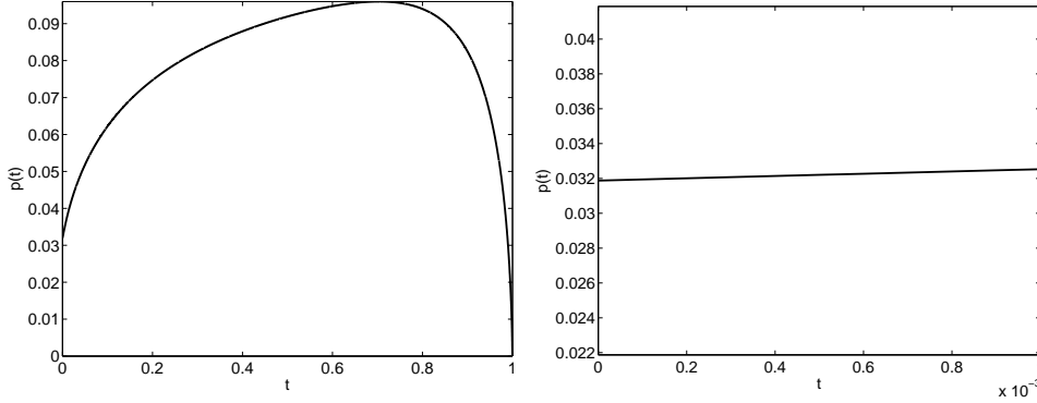
Figure 4: Numerical solution of (4.3), (4.4), (4.5) for a_0 = 1 , b_0 = 2 , \gamma = \frac{3}{2} . Left graph: p(t) , t \in [0, 1] ; Right graph: p(t) , t \in [0, 10^{-3}] .
