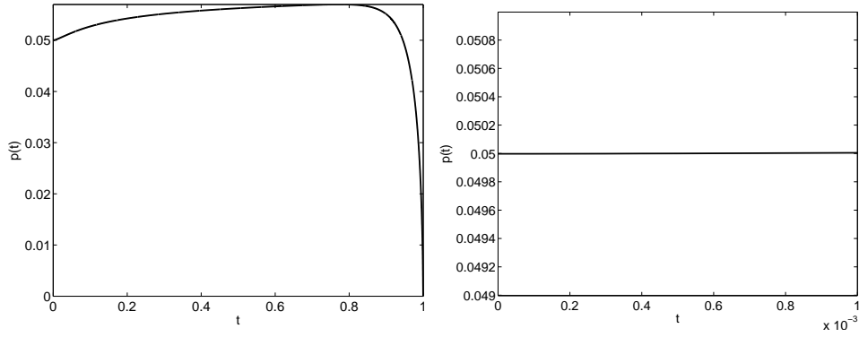
Figure 1: Numerical solution of (4.1), (4.2) for a_0 = 2 , b_0 = 3 , \gamma = 1.8 . Left graph: p(t) , t \in [0, 1] ; Right graph: p(t) , t \in [0, 10^{-3}] .
