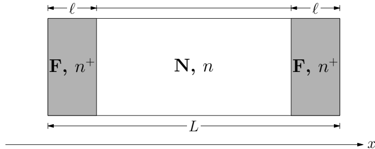
FIGURE 1. Geometry of the three-layer structure with ferromagnetic ( F ) highly doped ( n^+ ) source and drain regions and nonmagnetic ( N ) lowly doped ( n ) channel region.
