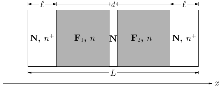
FIGURE 4. Geometry of the five-layer structure with ferromagnetic ( \mathbf{F}_1, \mathbf{F}_2 ) lowly doped ( n ) regions and nonmagnetic ( \mathbf{N} ) regions. The source and drain regions are highly doped ( n^* ), while the middle region is lowly doped.
