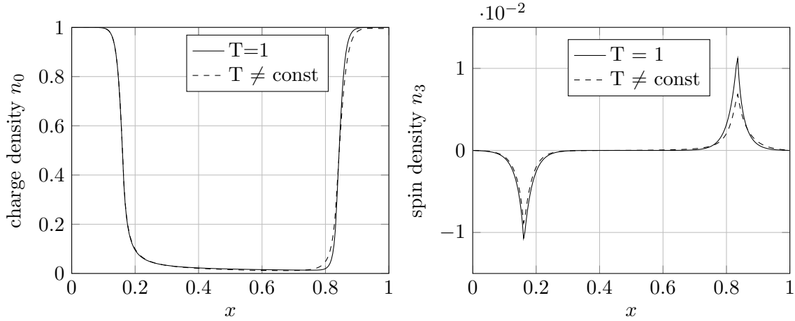
FIGURE 2. Charge density n_0 (left) and spin density n_3 (right) in the three-layer structure computed from the spin energy-transport model ( T \neq \text{const.} ) and from the corresponding spin drift-diffusion model ( T = 1 ).
