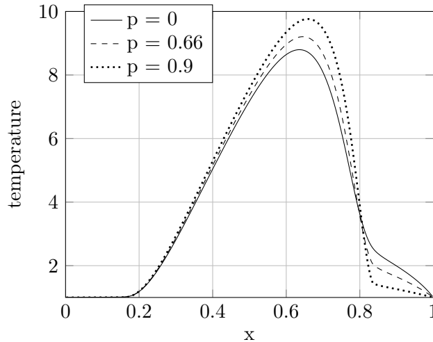
FIGURE 3. Temperature in the three-layer structure for various polarizations p .
