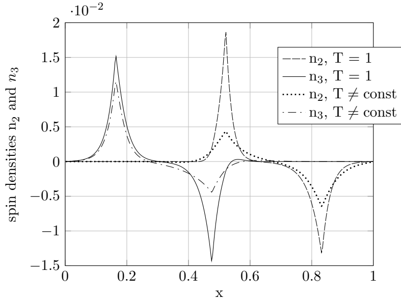
FIGURE 6. Spin density components n_2 and n_3 in the five-layer structure computed from the spin energy-transport model ( T \neq \text{const.} ) and from the corresponding spin drift-diffusion model ( T = 1 ).
