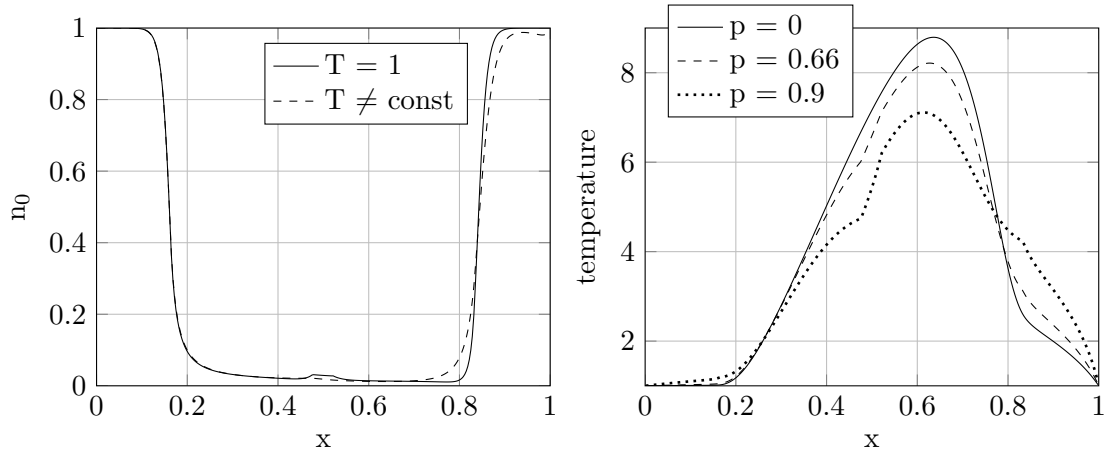
FIGURE 5. Charge density n_0 (left) and temperature T (right) in the five-layer structure.
