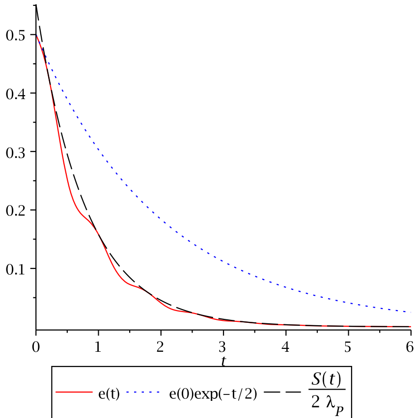
Figure 2.5: Entropy decay for the non-degenerate, non-symmetric Fokker-Planck equation (2.1) with \mathbf{D} = \text{diag}(1/4, 1) , \mathbf{C} = \begin{bmatrix} 1/4 & -4 \\ 4 & 1 \end{bmatrix} . Solid red curve: decay of the logarithmic entropy e_1(t) ; dotted blue: The estimate of the local decay rate from the standard entropy method is tangent at t = 0 ; dashed black: estimate of the global decay rate from the hypocoercive entropy method. (colors only online)
