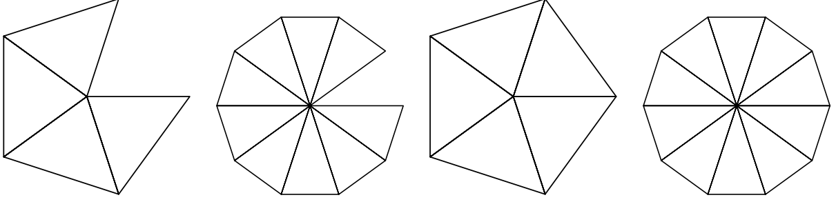
FIGURE 2. Reference patches \widehat{\omega}_N and \widehat{\omega}'_N in Lemma 10 for z \in \partial\Gamma and N = 4 as well as N = 9 resp. for z \notin \partial\Gamma and N = 5 as well as N = 10 (from left to right).
