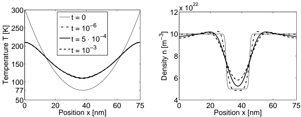
FIGURE 1. Periodic boundary conditions, case (i): Electron temperature (left) and electron density (right) at various times.
