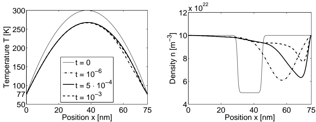
FIGURE 6. Case (ii), Dirichlet-Neumann boundary conditions: Electron temperature (left) and electron density (right) at various times.
