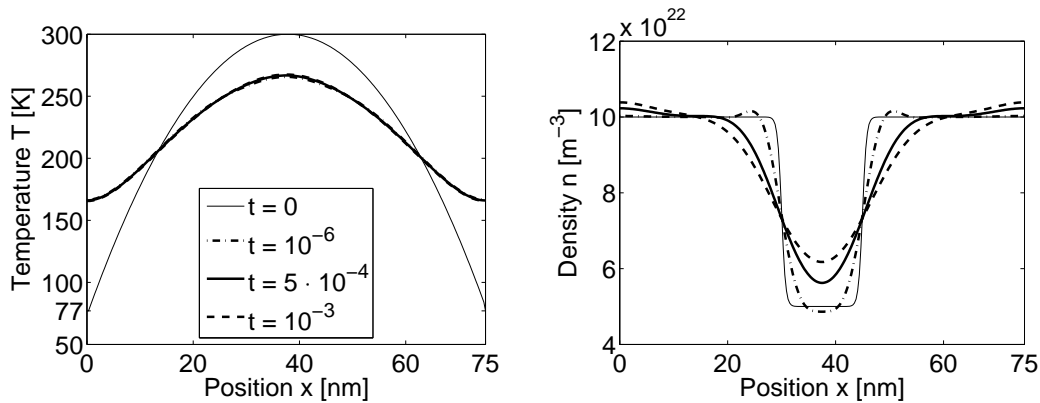
FIGURE 2. Periodic boundary conditions, case (ii): Electron temperature (left) and electron density (right) at various times.
