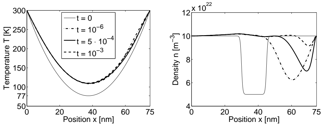
FIGURE 5. Case (i), Dirichlet-Neumann boundary conditions: Electron temperature (left) and electron density (right) at various times.
