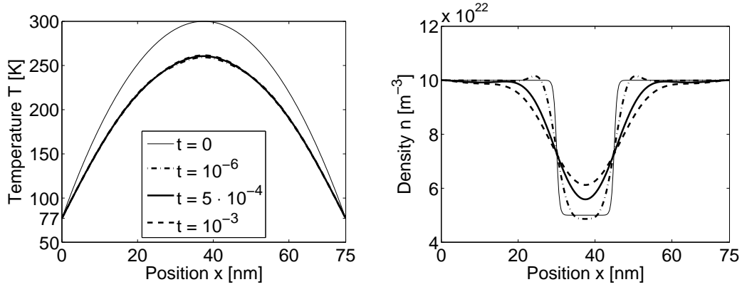
FIGURE 4. Dirichlet-Neumann boundary conditions, case (ii): Electron temperature (left) and electron density (right) at various times.
