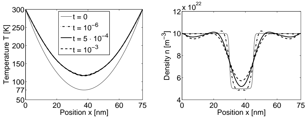
FIGURE 3. Dirichlet-Neumann boundary conditions, case (i): Electron temperature (left) and electron density (right) at various times.
