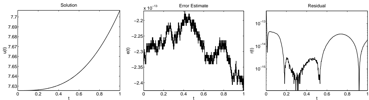
Figure 19: Problem (3.45): The numerical solution, the error estimate and the residual for \lambda = 0.69901190254861 .
