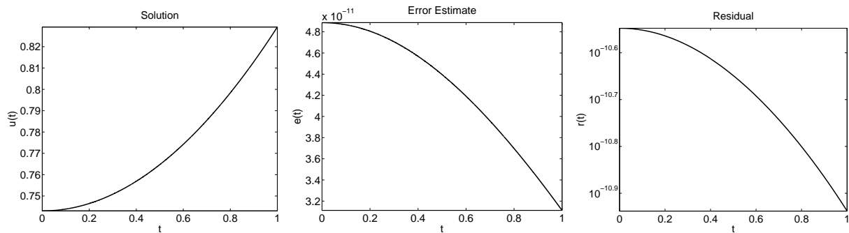
Figure 7: Problem (3.42): The numerical solution, the error estimate and the residual for \alpha = 1 , \beta = 1 and \lambda = 0.15 . The associated root is x_2 .
