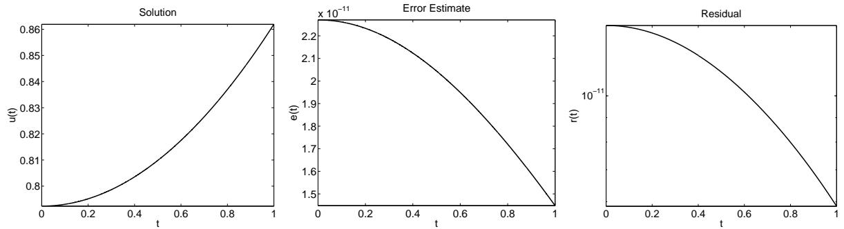
Figure 4: Problem (3.41): The numerical solution, the error estimate and the residual for \alpha = 1 , \beta = 1 and \lambda = (4/9)(3/(3\alpha + 4\beta))^{3/2} .
