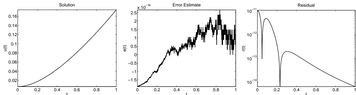
Figure 8: Problem (3.41): The numerical solution, the error estimate and the residual for \alpha = 5 , \beta = 0.5 and \lambda = 0.05 . The associated root is x_1 .
