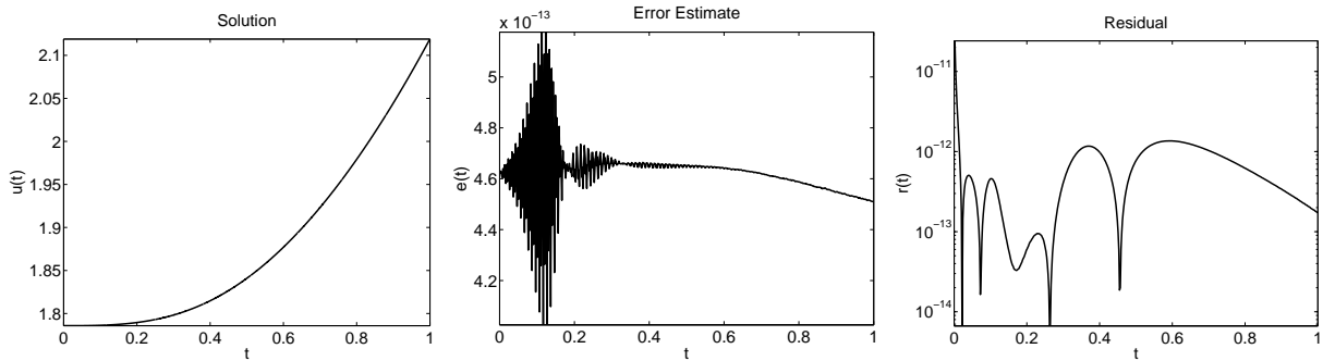
Figure 27: Problem (3.45): The numerical solution, the error estimate and the residual for \lambda = 1.84240837502548 .
