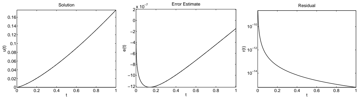
Figure 13: Problem (3.43): The numerical solution, the error estimate and the residual for \alpha = 5 , \beta = 0.5 and \lambda = (4/9)(3/(3\alpha + 4\beta))^{3/2} .
