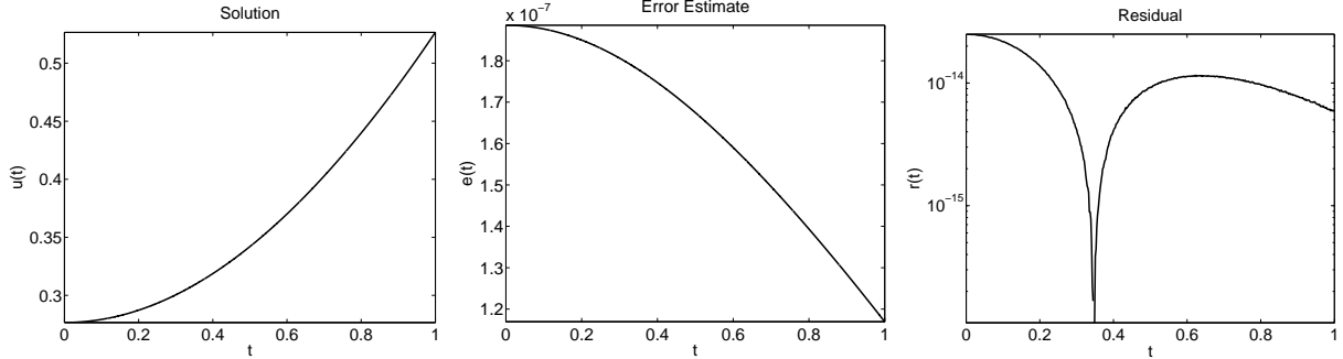
Figure 10: Problem (3.41): The numerical solution, the error estimate and the residual for \alpha = 1, \beta = 1 and \lambda = 0.28049410745840 .
