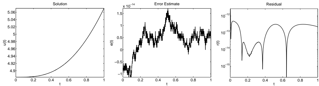
Figure 23: Problem (3.45): The numerical solution, the error estimate and the residual for \lambda = 1.42604644036221 .
