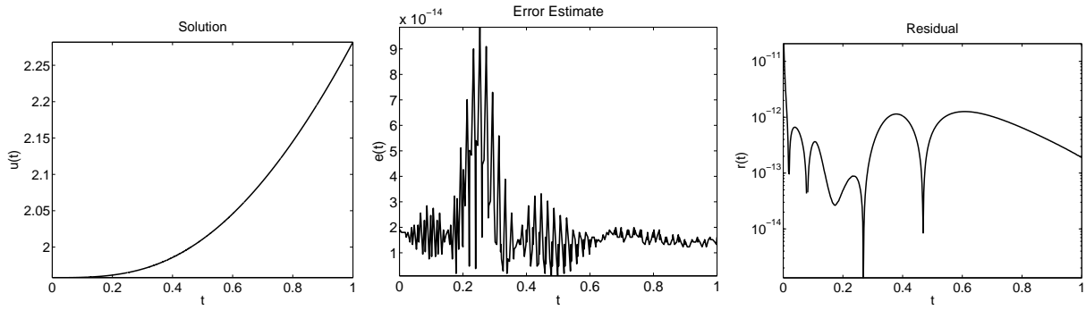
Figure 26: Problem (3.45): The numerical solution, the error estimate and the residual for \lambda = 1.84416811671110 .
