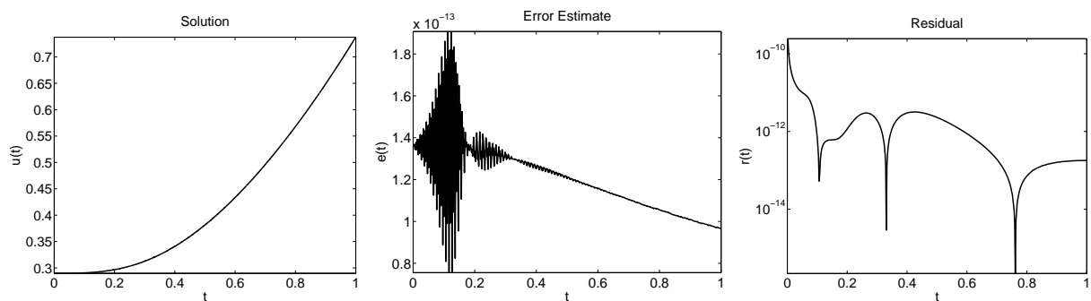
Figure 24: Problem (3.45): The numerical solution, the error estimate and the residual for \lambda = 1.42139222684689 .
