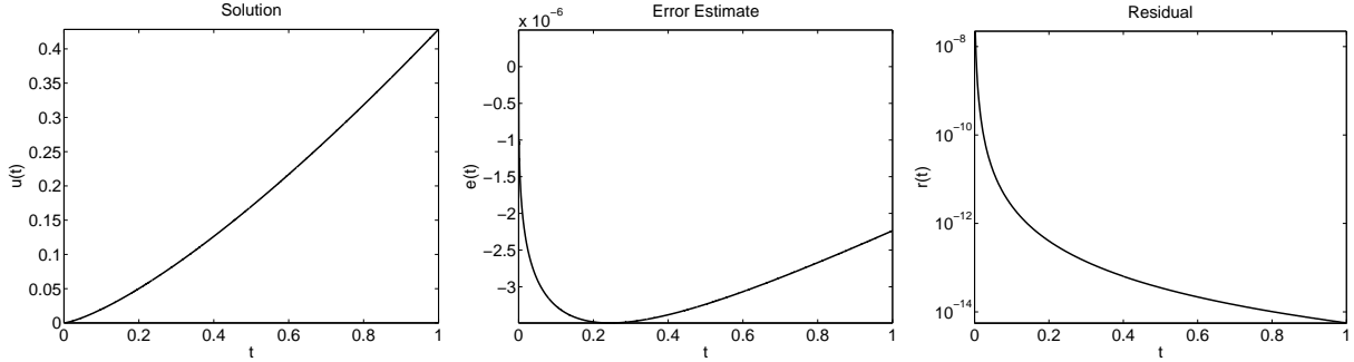
Figure 12: Problem (3.43): The numerical solution, the error estimate and the residual for \alpha = 1 , \beta = 1 and \lambda = (4/9)(3/(3\alpha + 4\beta))^{3/2} .
