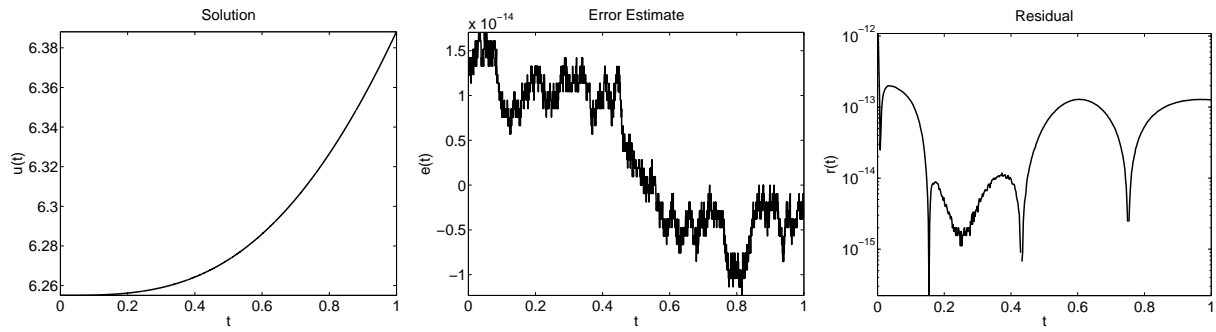
Figure 20: Problem (3.45): The numerical solution, the error estimate and the residual for \lambda = 1.08259965025194 .
