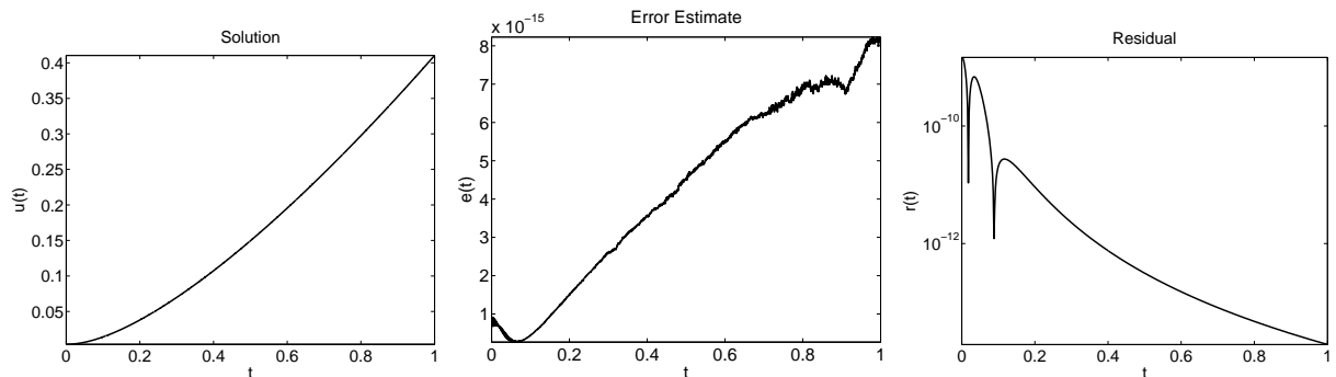
Figure 6: Problem (3.41): The numerical solution, the error estimate and the residual for \alpha = 1 , \beta = 1 and \lambda = 0.15 . The associated root is x_1 .
