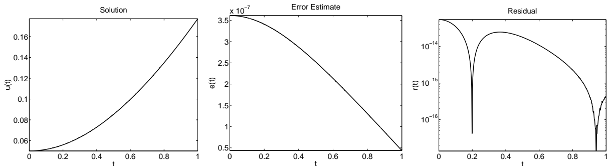
Figure 11: Problem (3.41): The numerical solution, the error estimate and the residual for \alpha = 5, \beta = 0.5 and \lambda = 0.06608546529011 .
