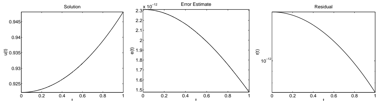
Figure 2: Problem (1.7): The numerical solution, the error estimate and the residual for \alpha = 1, \beta = 1 and \lambda = 0.05 .
