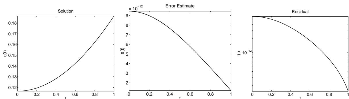
Figure 9: Problem (3.42): The numerical solution, the error estimate and the residual for \alpha = 5 , \beta = 0.5 and \lambda = 0.05 . The associated root is x_2 .
