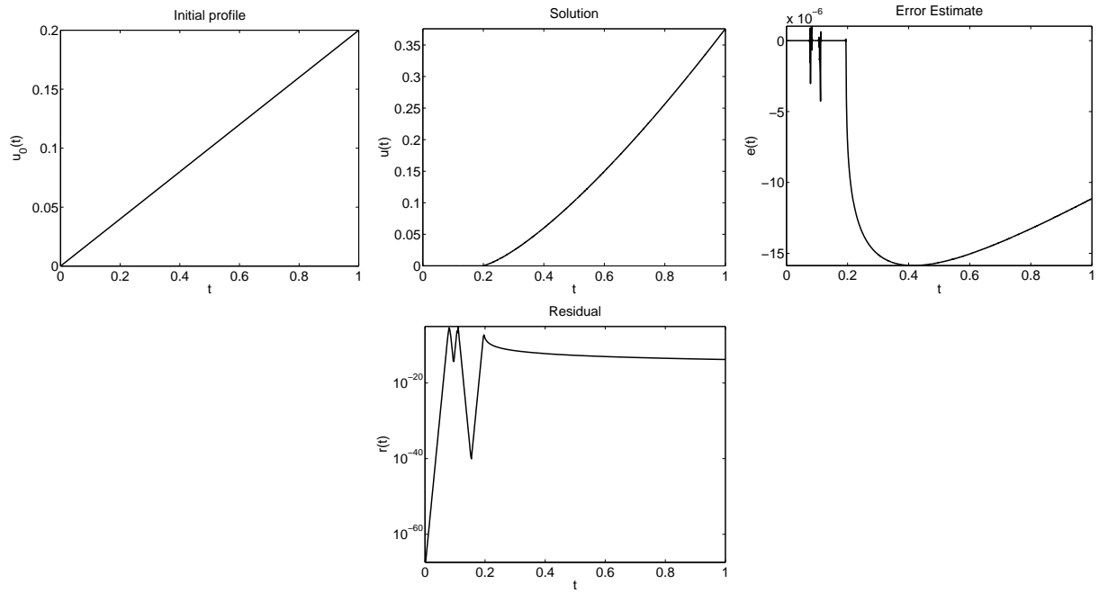
Figure 14: Problem (3.43): The initial profile, the numerical solution, the error estimate and the residual for \alpha = 1 , \beta = 1 and t_1 = 0.2 .
