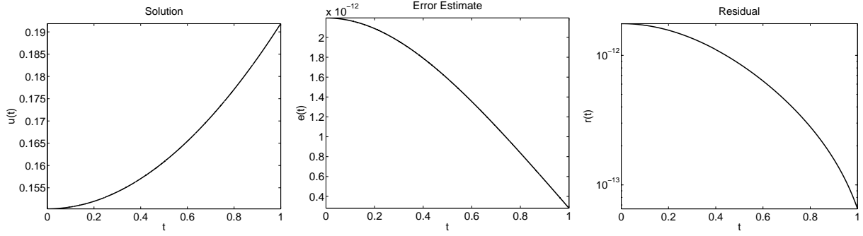
Figure 5: Problem (3.41): The numerical solution, the error estimate and the residual for \alpha = 5 , \beta = 0.5 and \lambda = (4/9)(3/(3\alpha + 4\beta))^{3/2} .
