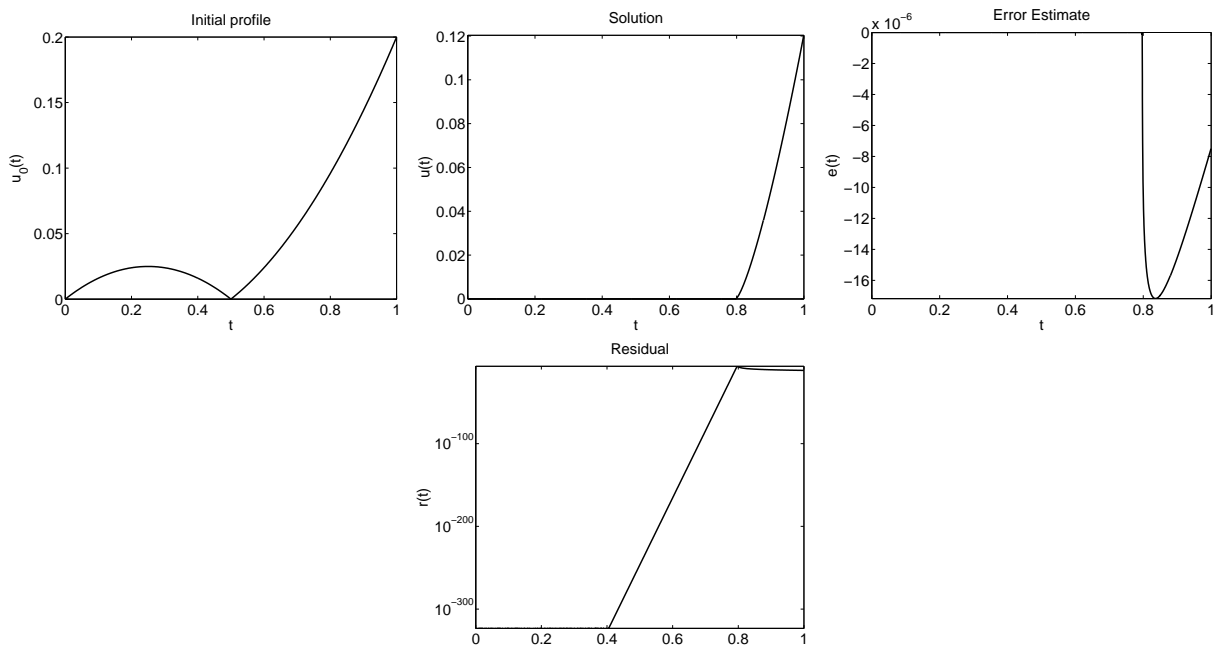
Figure 17: Problem (3.43): The initial profile, the numerical solution, the error estimate and the residual for \alpha = 5 , \beta = 0.5 and t_1 = 0.8 .
