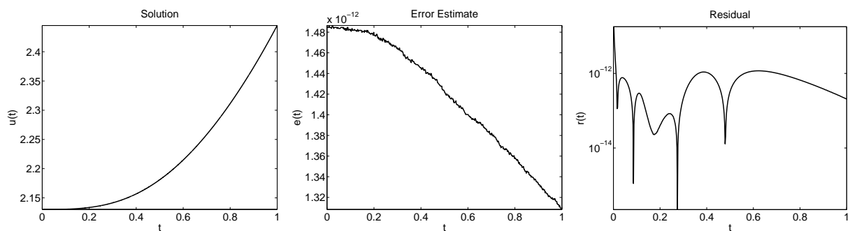
Figure 25: Problem (3.45): The numerical solution, the error estimate and the residual for \lambda = 1.84118395344504 .
