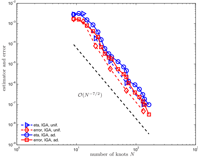
FIGURE 5.2. Experiment with smooth solution on circle geometry from Section 5.2. Error and estimator are plotted versus the number of knots N .
