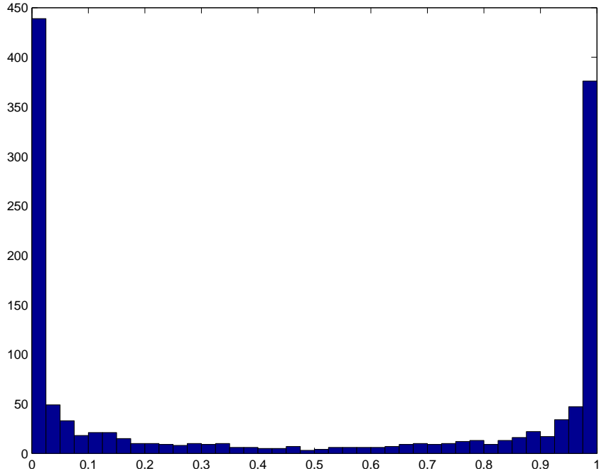
FIGURE 5.7. Experiment with singular solution on slit from Section 5.4. Histogram of number of knots over the parameter domain.
