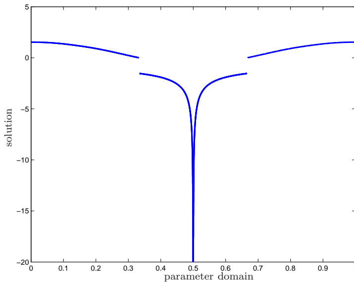
FIGURE 5.3. Experiment with singular solution on pacman geometry from Section 5.3. The singular solution \phi \circ \gamma is plotted on the parameter interval, where 0.5 corresponds to the origin, where \phi is singular.
