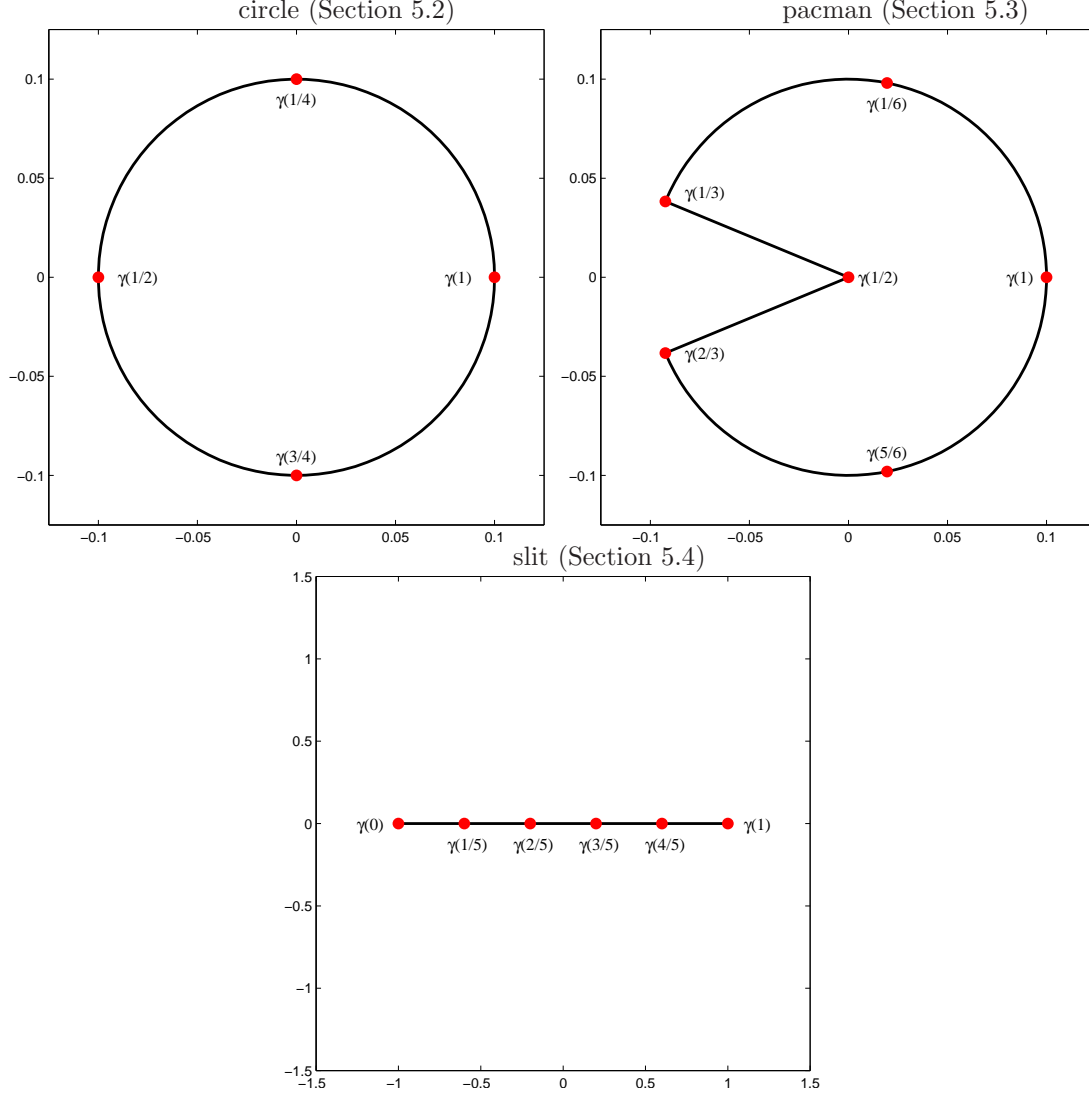
FIGURE 5.1. Geometries and initial nodes for the experiments from Section 5.2–5.4.
