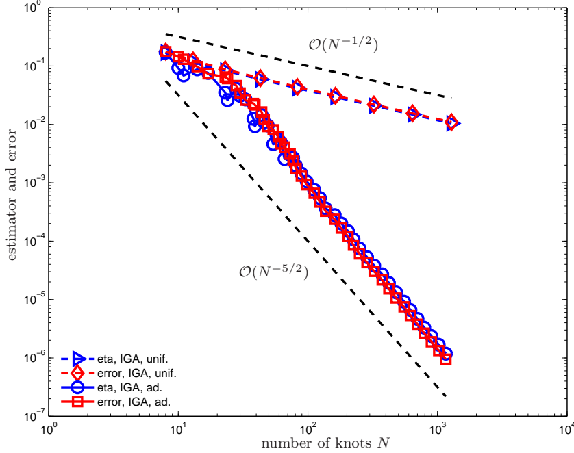
FIGURE 5.6. Experiment with singular solution on slit from Section 5.4. Error and estimator are plotted versus the number of knots N .
