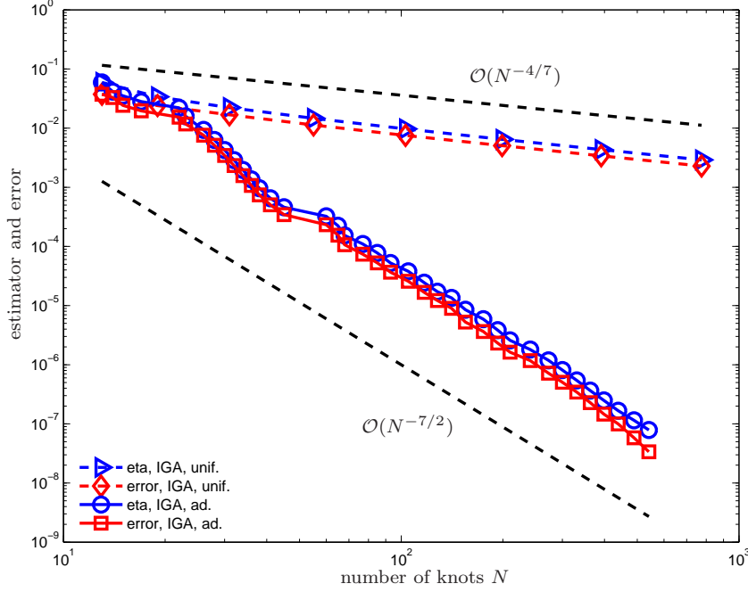
FIGURE 5.4. Experiment with singular solution on pacman geometry from Section 5.3. Error and estimator are plotted versus the number of knots N .
