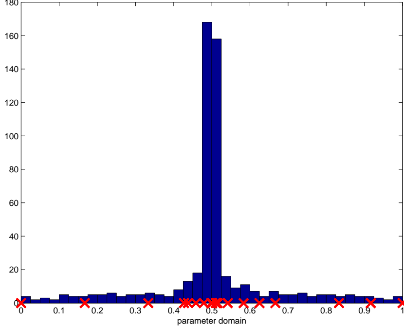
FIGURE 5.5. Experiment with singular solution on pacman geometry from Section 5.3. Histogram of number of knots over the parameter domain. Knots with maximal multiplicity p + 1 = 3 are marked.
