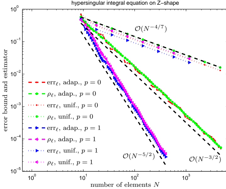
FIGURE 2. Hyper-singular integral equation from Section 7.1 on the Z-shaped domain, sketched in Figure 1. Uniform mesh-refinement leads to a suboptimal convergence \mathcal{O}(N^{-4/7}) for both p = 0 and p = 1 , whereas the adaptive strategy recovers the optimal convergence \mathcal{O}(N^{-(3/2+p)}) .
