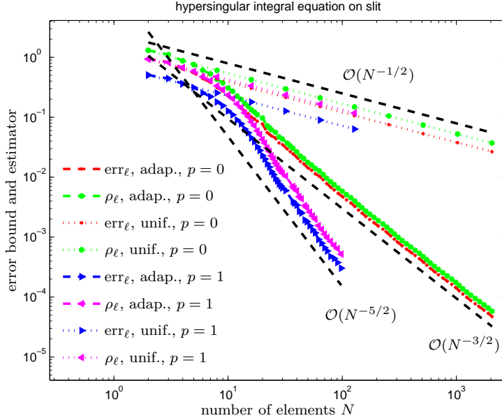
FIGURE 3. Hyper-singular integral equation from Section 7.2 on the slit \Gamma := (-1, 1) \times \{0\} . Uniform mesh-refinement leads to a suboptimal convergence \mathcal{O}(N^{-1/2}) for both p = 0 and p = 1 , whereas the adaptive strategy recovers the optimal convergence \mathcal{O}(N^{-(3/2+p)}) .
