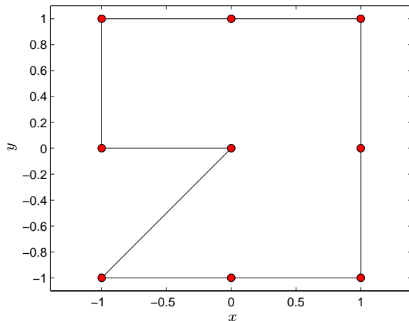
FIGURE 1. Z-shaped domain \Omega with boundary \Gamma = \partial\Omega and initial triangulation of \Gamma into 9 boundary elements for the numerical experiment from Section 7.1.
