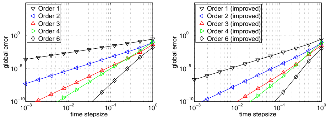
Figure 1: Linear Schrödinger equation: Global errors versus time stepsizes for different splitting methods (left) of orders p = 1, 2, 3, 4, 6 and associated improved approximations (right) of orders p + 1 resulting from the a posteriori local error estimators (7).
