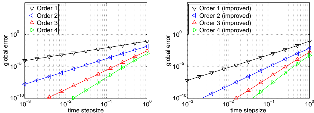
Figure 2: Parabolic equation: Global errors versus time stepsizes for different splitting methods (left) of orders p = 1, 2, 3, 4 and associated improved approximations (right) of orders p + 1 resulting from the a posteriori local error estimators (7).
